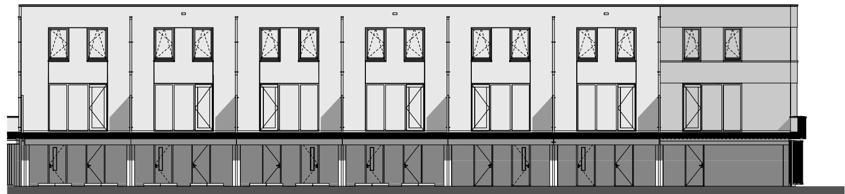
Binnengevel West
